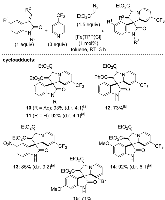
Scheme 5. Synthesis of tetrahydroindolizidines from various 3-alkenyloxindoles. [a] The diastereomeric ratio was determined by NMR analysis. [b] Synthesized from either ( E )-3-phenacylideneoxindole or ( Z )-3-phenacylideneoxindole.
